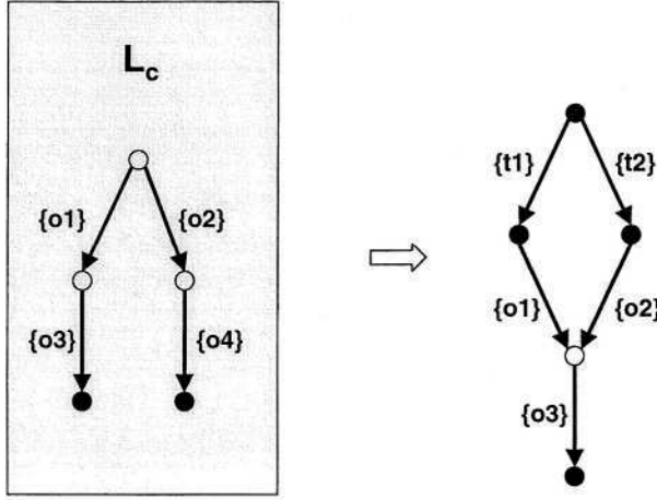
Fig. 12. In general two words v = \{t_2\}\{o_2\} \notin M_{blocking}^k and w = \{t_1\}\{o_1\} \in M_{blocking}^k can have the same follower state in an automaton A recognizing L_{safe} . For the automaton G implementing the nonblocking algorithm however we require that one can distinguish between “blocking-states” and “not blocking-states”. Such states can be splitted appropriately by synchronizing A with an automaton recognizing \lambda_{T \cup I}^{-1}(L_c) .
