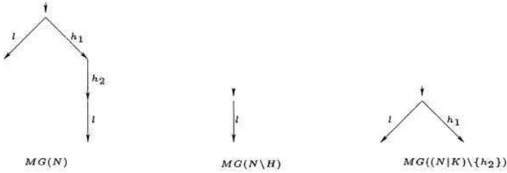
Fig. 4. The marking graphs of the net systems N , NH and (N \mid K) \setminus \{h_2\} .
