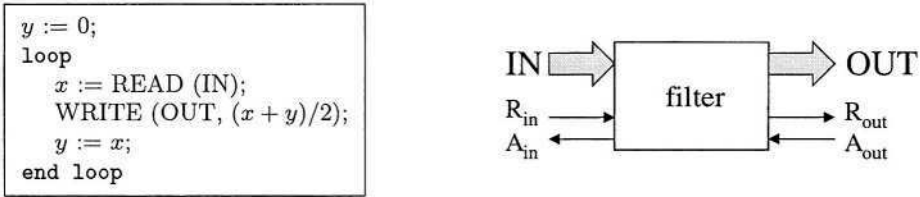
Fig. 2. High-level specification of a filter.
