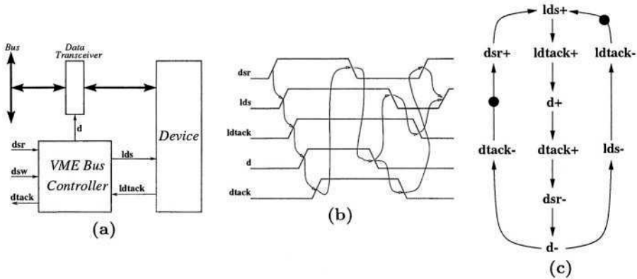
Fig. 7. VME bus controller: interface (a), the timing diagram for the read cycle (b) and the STG for the read cycle (c).
