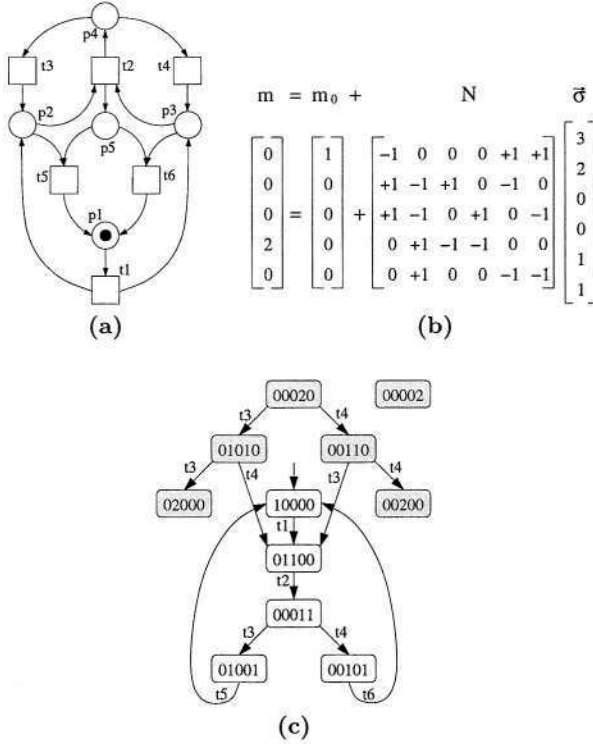
Fig. 16. A Petri net (a), a spurious solution M = (00020)^T (b), and the potential reachability graph (c).
