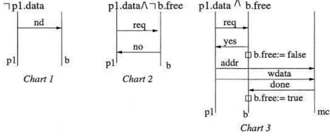
Fig. 3. Distributed nature of choice in a net transition
