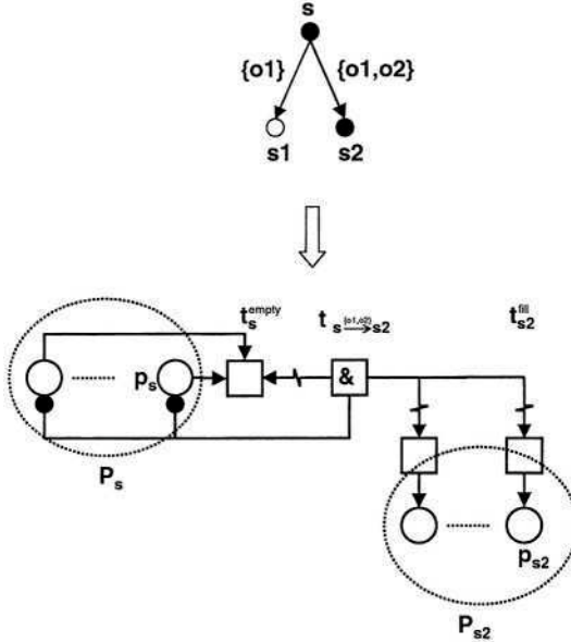
Fig. 16. For clearness we model only the transition s \xrightarrow{\{o1, o2\}} s_2 of the above behavior (the black states). The transition t_{s \xrightarrow{\{o1, o2\}} s_2} simulates the edge s \xrightarrow{\{o1, o2\}} s_2 . t_{s \xrightarrow{\{o1, o2\}} s_2} synchronizes t_s^{empty} to empty the marking P_s , and synchronizes exactly the transitions t_p^{fill} with p \in P_{s_2} (observe in particular p_s \in P_s and p_{s_2} \in P_{s_2} ). Moreover t_{s \xrightarrow{\{o1, o2\}} s_2} tests the places in P_s to be marked. The event arc connections to input and output transitions are omitted (see Figure 17).
