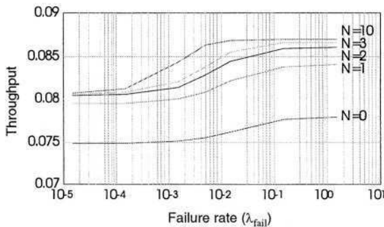
Fig. 4. Performance evaluation of the cell in Fig. 1 with respect to failure rate.
