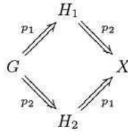
Fig. 13. Local Church-Rosser Property
