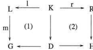
Fig. 7. Graph Transformation with Pushouts (1) and (2)
