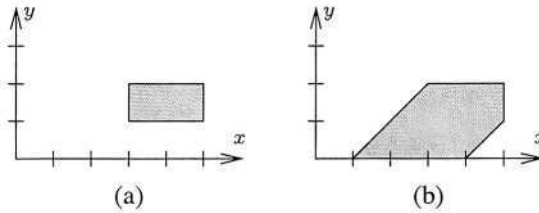
Fig. 12. Applying \text{down} to a zone.
