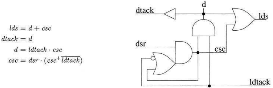
Fig. 13. Logic equations and implementation of the VME bus controller.
