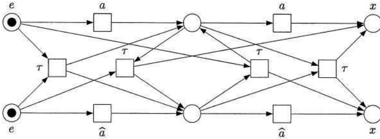
Fig. 4. Net for a.a.\text{nil} \mid \hat{a}.\hat{a}.\text{nil} .
