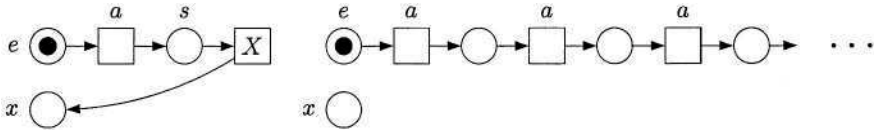
Fig. 13. Nets for X \stackrel{\text{df}}{=} a; X : the body and solution.
