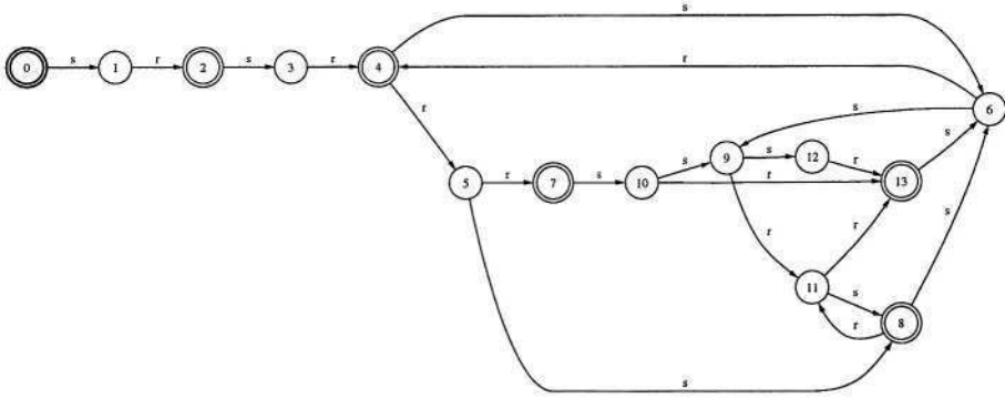
Fig. 11. FSA showing erroneous sequences of send and receive primitives for the Stop-and-Wait protocol operating over a lossless reordering medium.
