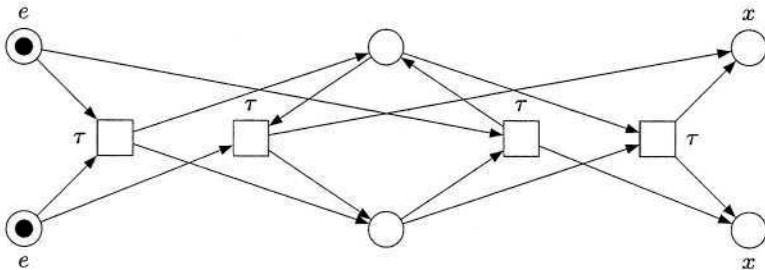
Fig. 6. Net for (a.a.nil \mid \hat{a}.\hat{a}.nil)\backslash a .
