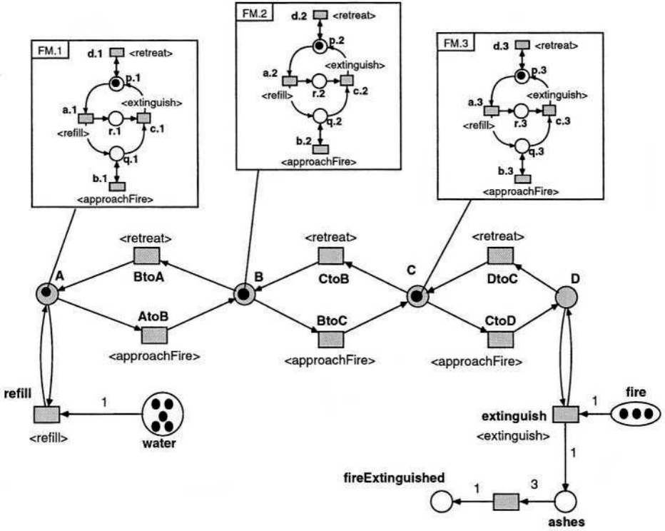
Fig. 12. Elementary object net for parallel fire extinction
