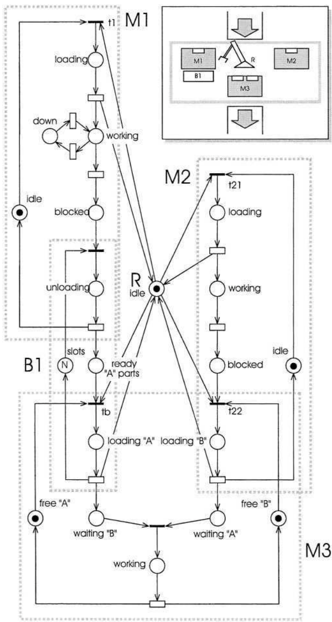
Fig. 1. An autonomous place/transition system that formally describes the logic behaviour of a manufacturing cell.
