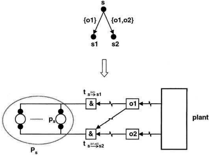
Fig. 17. The transition t_{s \rightarrow s_2}^{\{o_1, o_2\}} simulates the edge s \xrightarrow{\{o_1, o_2\}} s_2 . It is therefore synchronized by the output transitions o_1 and o_2 . The occurrence of o_1 together with o_2 synchronizes also t_{s \rightarrow s_1}^{\{o_1\}} , since t_{s \rightarrow s_1}^{\{o_1\}} is also enabled under P_s . The occurrence of o_1 without o_2 only synchronizes t_{s \rightarrow s_1}^{\{o_1\}} . For clearness the connections to empty- and fill-transitions and places in the follower marking are omitted (see Figure 16), but observe that this implies p_{s_1} \in P_{s_1} \subset P_{s_2} . (see also Figure 20).
