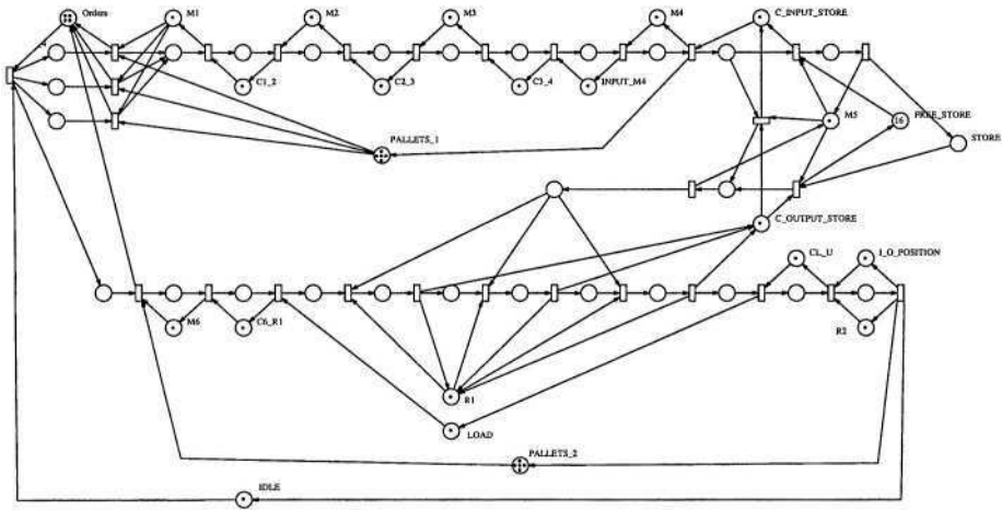
Fig. 28. A non-sequential RAS modelling the assembly of a product made of three complete cylinders and a base.
