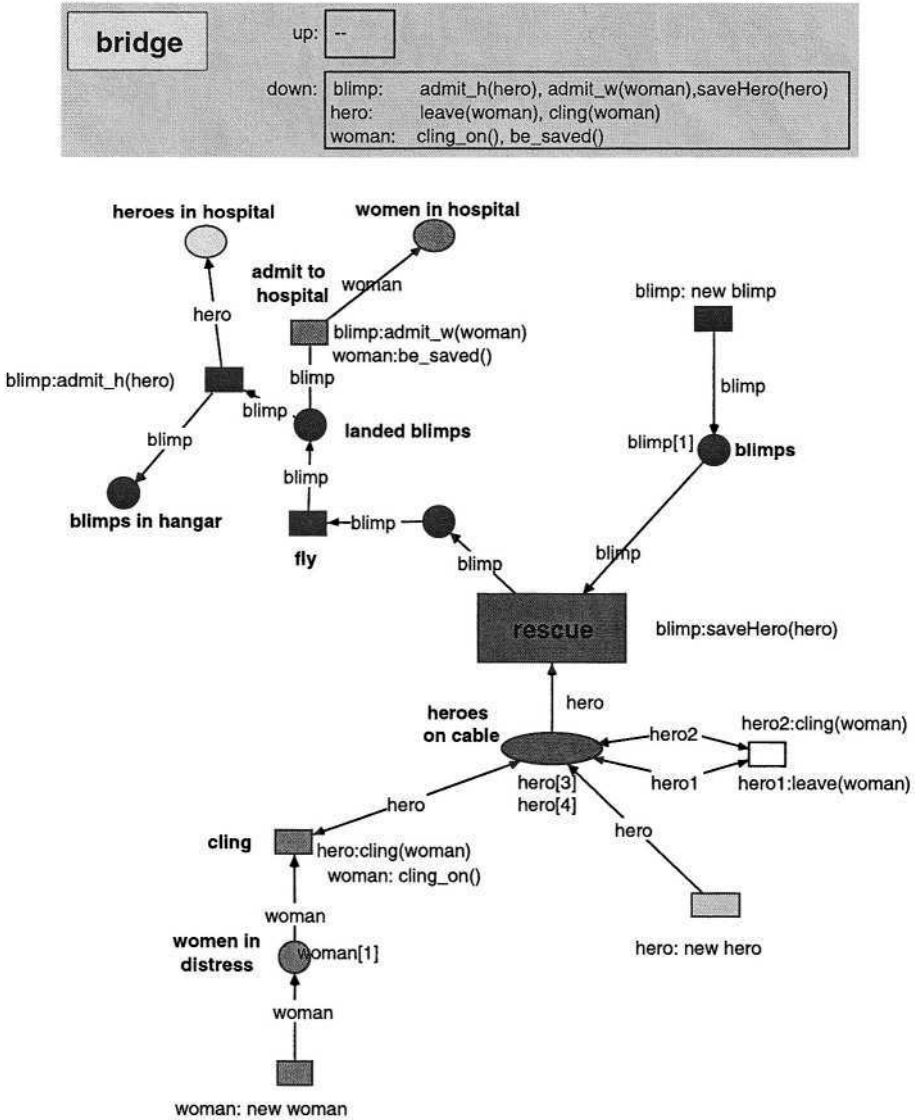
Fig. 26. The garbage can object system: bridge
