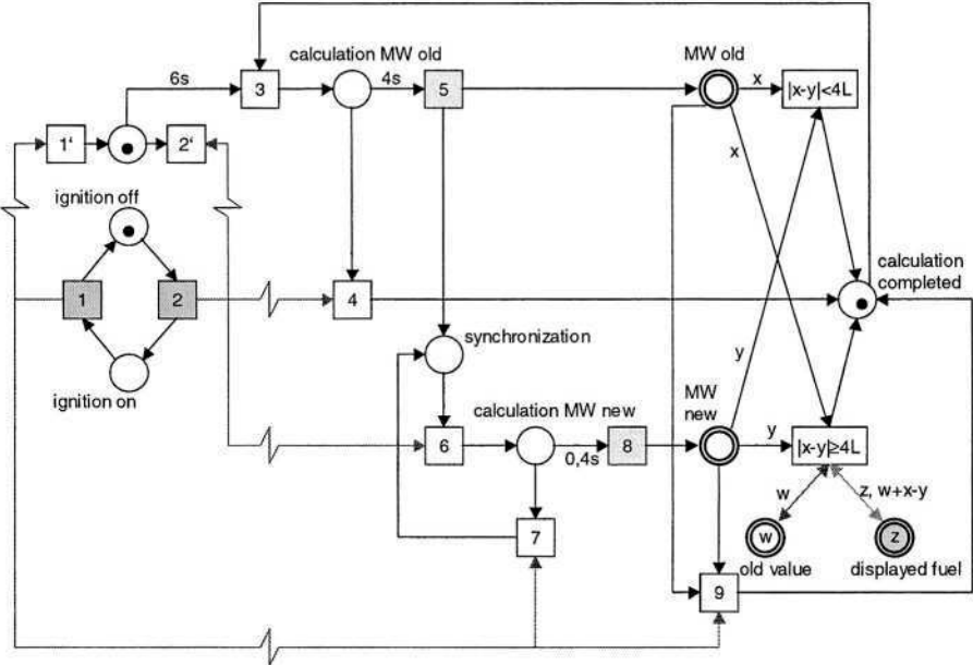
Fig. 13. Signal net model of the fuel gauge while the ignition is off
