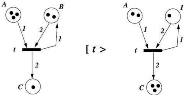
Fig. 17. Transition Firing as Token Game
